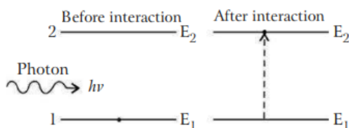
Fig. 1. Induced or stimulated absorption. Source: Physical Optics and Lasers by R.K. Agrawal
