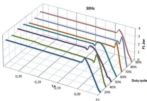
Fig. 4. Pressure drop in the left chamber of the pneumatic cylinder at a frequency of 30 Hz and a different duty cycle.
