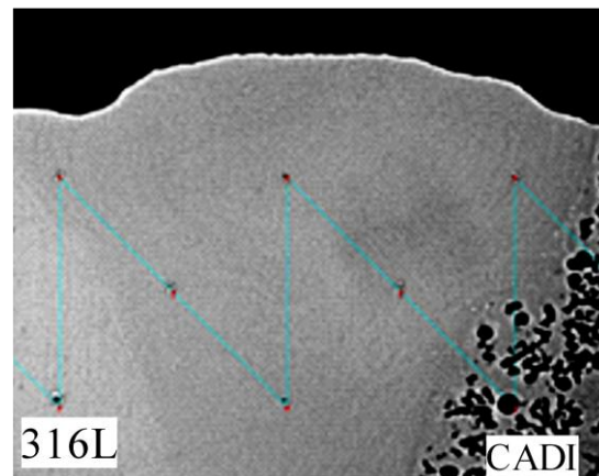
Fig. 2 Vickers microhardness measurement of specimen No. 4.
