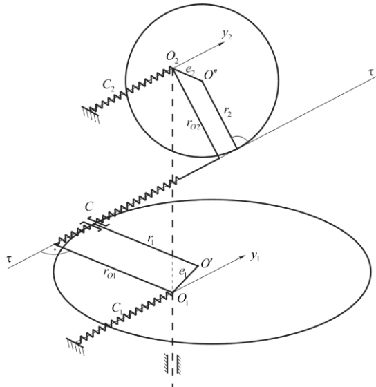
Fig. 3. The dynamic model of the single-stage bevel gear
