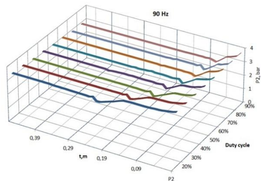
Fig. 13. Pressure washout in the right chamber of the pneumatic cylinder at a frequency of 90 Hz and a different duty cycle.
