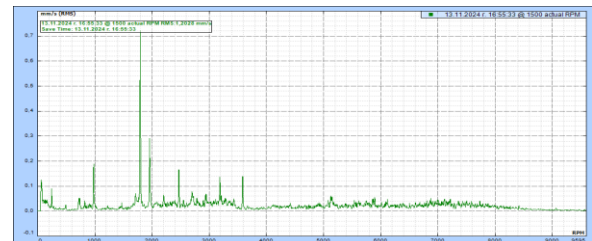
Fig. 7-a Azimuth thruster oscillation spectrum starboard side vertical
