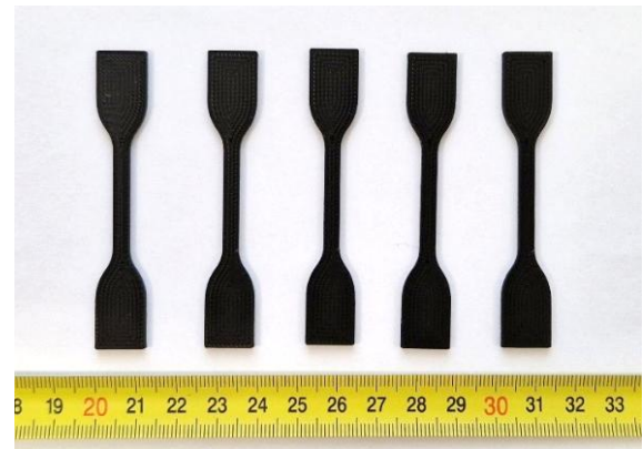
Fig. 2. ISO 527-5A compliant tensile test specimens produced by FFF.
