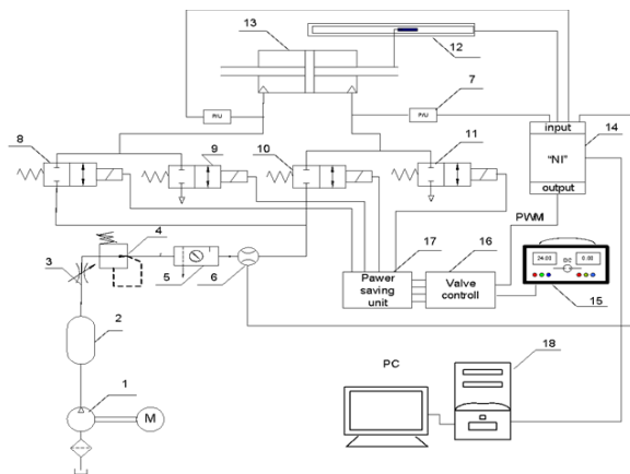
Fig. 2. Schematic Diagram of the High-Speed Pneumatic On/Off Valve with PWM Control
