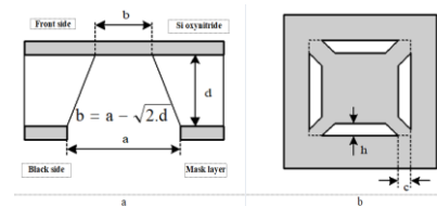
Fig. 1. Etching of membranes:
