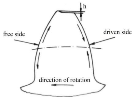
Fig. 1. Material displacement in the process of tooth machining by calibration.
