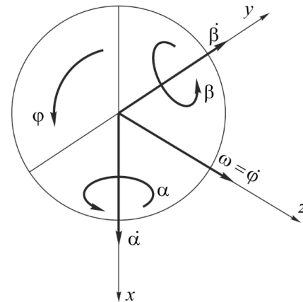
Fig. 3. The propeller is represented as a disk
