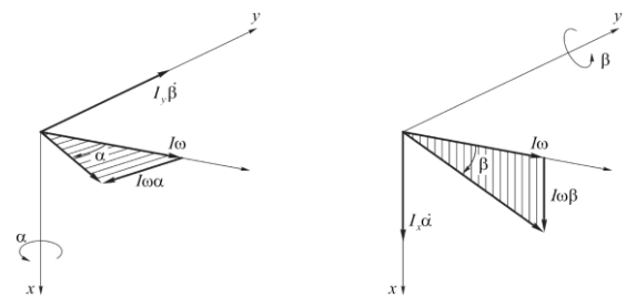
Fig. 4-a. Projection of the kinetic moment along the x and y axes
