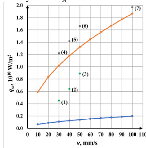
Fig. 1. Graphs of the dependence of the critical power density of melting and evaporation on the speed for AISI 316 steel for the laser marking process.
