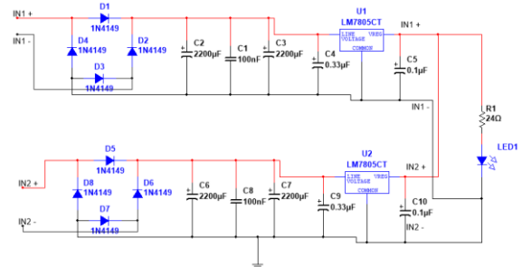
Fig. 12. Principle electrical scheme of parallel connection of two sources.
