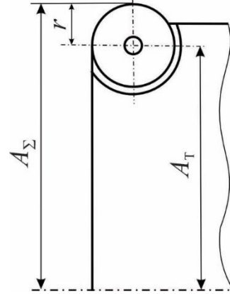
Fig. 5. Dimensioning round insert
