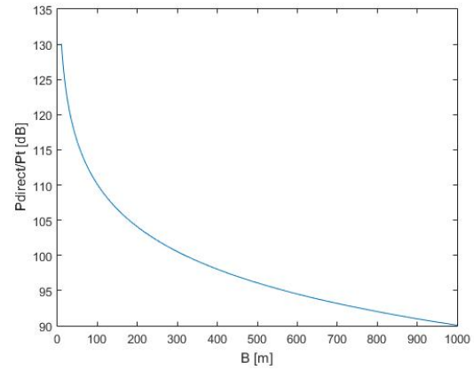
Fig. 4. Direct channel to target signal ratio.
