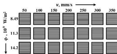
Fig. 3. Designed matrix of the experiments for laser marking of CuZn samples.
