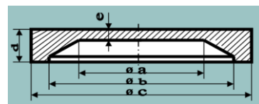
Fig. 4. Flat round membrane with one-sided stoppers
