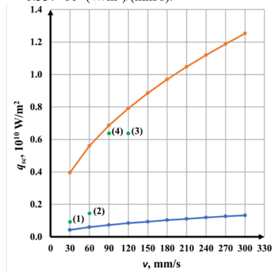
Fig. 3. Graphs of the dependence of the critical power density of melting and evaporation on the speed for AISI 316 steel for the laser welding process
