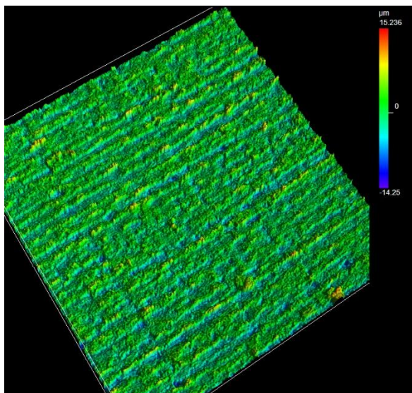
Fig. 8. Laser made hydrophobic surface structure under microscope.
