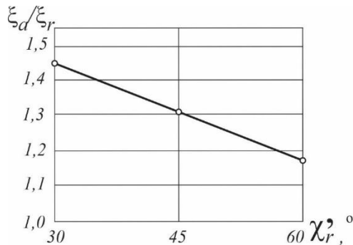
Fig. 6. Dependence of the ratio of the transmission coefficients \xi_a and \xi_r on the auxiliary setting angle
