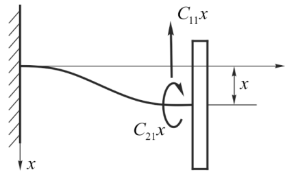
Fig. 5-b the elastic constants of the cantilever shaft. When specifying a displacement x
