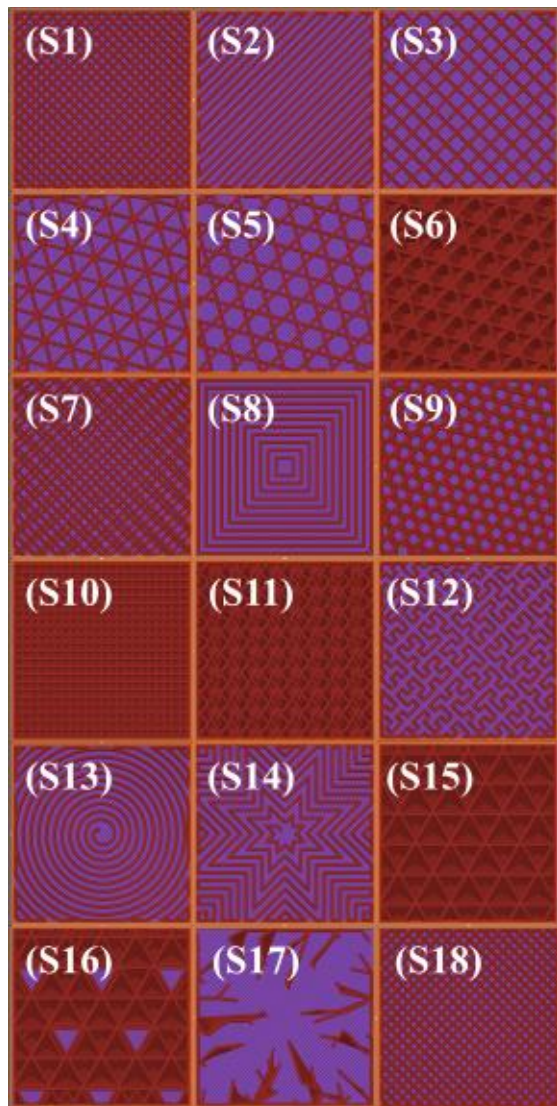
Fig. 1. Visualization of the eighteen infill patterns tested in this study: Rectilinear (S1), Aligned Rectilinear (S2), Grid (S3), Triangles (S4), Stars (S5), Cubic (S6), Line (S7), Concentric (S8), Honeycomb (S9), 3D Honeycomb (S10), Gyroid (S11), Hilbert curve (S12), Archimedean Chords (S13), Octagram Spiral (S14), Adaptive Cubic (S15), Support Cubic (S16), Lightning (S17) and Zig Zag (S18).
