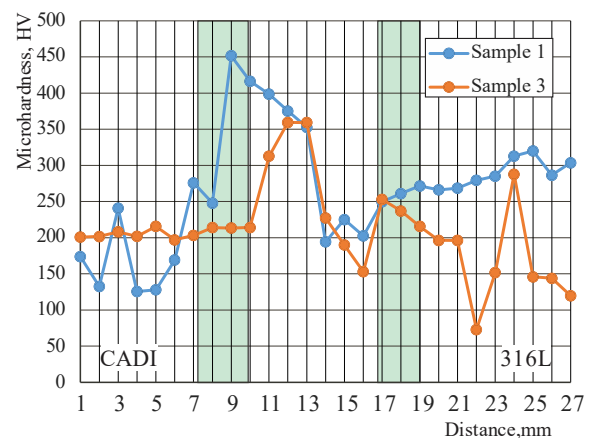
Fig. 3 Measured microhardness of electron beam welded samples with Beam current I_b=10\text{mA} .
