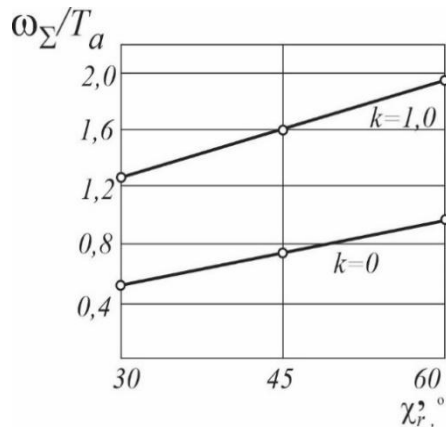
Fig. 7. Dependence of the ratio (\omega_\Sigma)/T_a on the auxiliary setting angle \chi'_r
