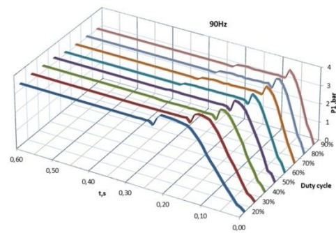
Fig. 12. Pressure drop in the left chamber of the pneumatic cylinder at a frequency of 90 Hz and a different duty cycle.
