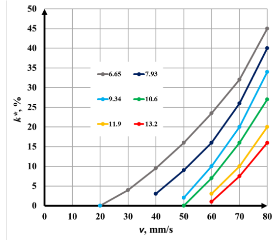
Fig. 6. Graphs of the dependence of contrast on speed for white (light) marking.
