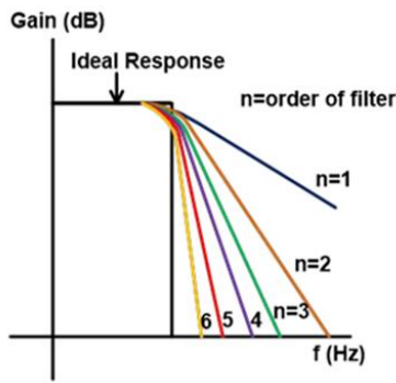
Fig. 2. Frequency response of the Butterworth filter for different filter orders.
