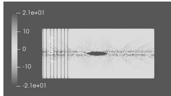
Fig. 9. Reconstructed Y- Velocity.
