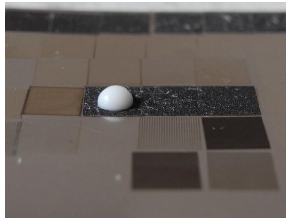
Fig. 5. Milk droplet on laser made hydrophobic surface.
