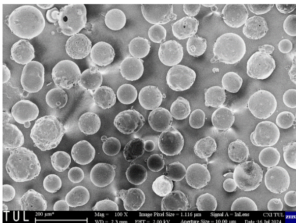
Fig. 1. Image of the cenospheres used.
