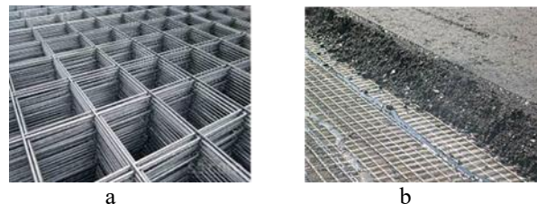
Fig. 5. Welded wire mesh (a) and its use in road construction (b).
