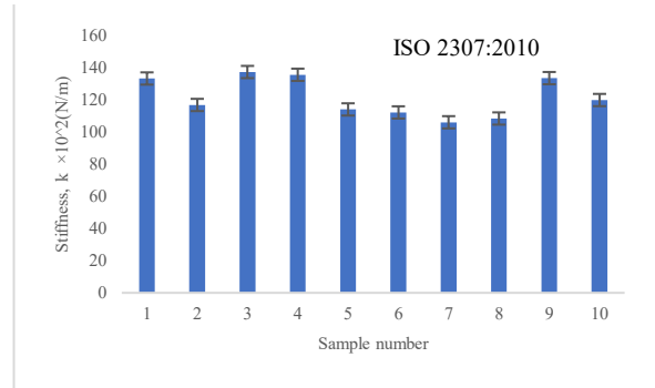
Fig. 5. Comparison graph of the stiffness values of the ten samples.
