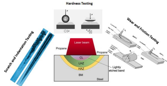
Fig. 10. Types of methods for mechanical and tribological analysis of laser hardened area
