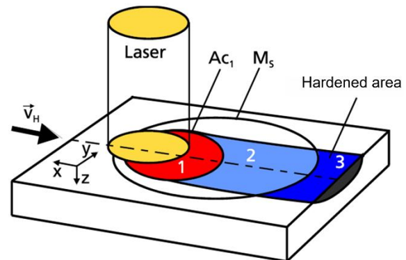
Fig.2. Principle scheme of laser hardening: V_H - the speed at which the laser beam moves; area (1) austenite structure; area (2) - austenite is supercooled; area (3) martensitic structure formation.
