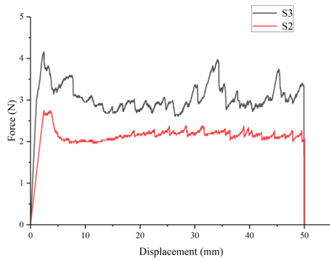
Fig. 3. Representative force displacement curves from T-peel testing of the nanofibre-laminated textiles of groups S2 and S3.
