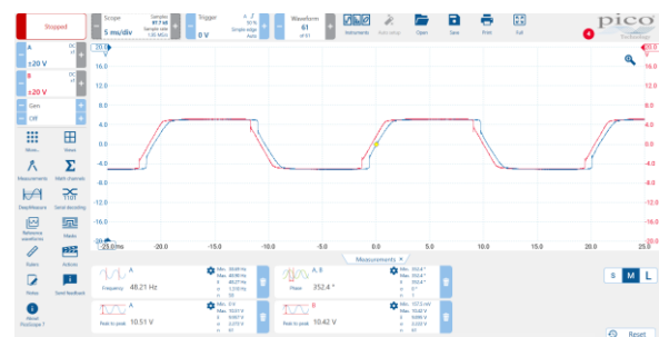
Fig. 13. Oscilloscope showing the changes in the generated voltage fluctuations (with diode bridges and load at parallel circuits).
