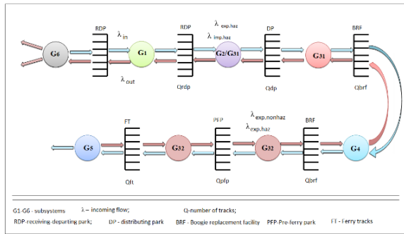
Fig.1 Structural diagram of the Ferry Complex - Varna as a QT system
