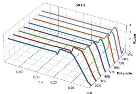
Fig. 8. Pressure drop in the left chamber of the pneumatic cylinder at a frequency of 50 Hz and a different duty cycle.
