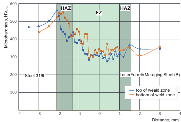
Fig. 7. Vickers microhardness in two parallel lines: the first was located at a distance of 1mm from the surface of the weld, and the second (bottom of weld zone) - at a distance of 3mm from the first.
