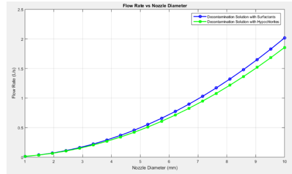
Fig. 1. Flow rate of decontamination solutions versus nozzle diameter.
