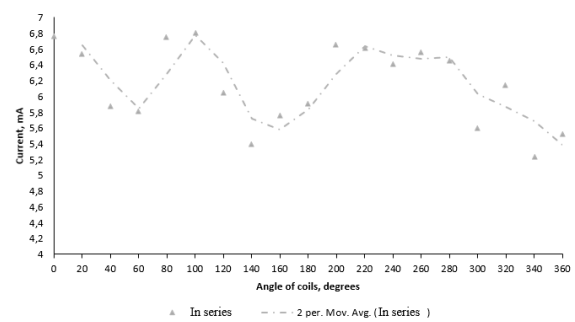
Fig. 11. The dependence of the current of two sources connected in series to the phase.
