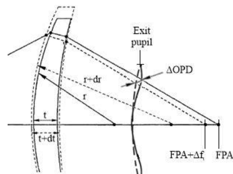
Fig. 1. Lens with thermal deformation.
