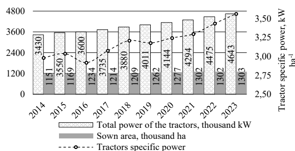
Fig. 3. Changes in the total capacity, specific capacity and sown area of agricultural crops of the tractor fleet in 2014-2023.
