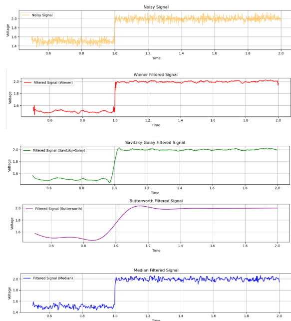
Fig. 4. Comparative presentation of simulated filter results.
