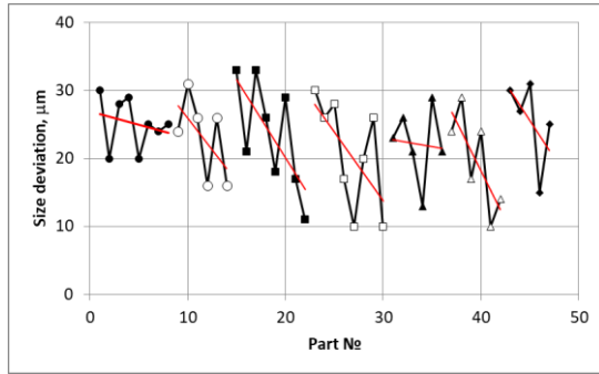
Fig. 3. Scatter diagram of the process of clean boring of a batch of cylindrical bushings with the application of an analytical method for dimension sub-tuning
