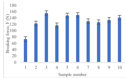
Fig. 3. Comparison graph of the values of breaking force of the ten samples
