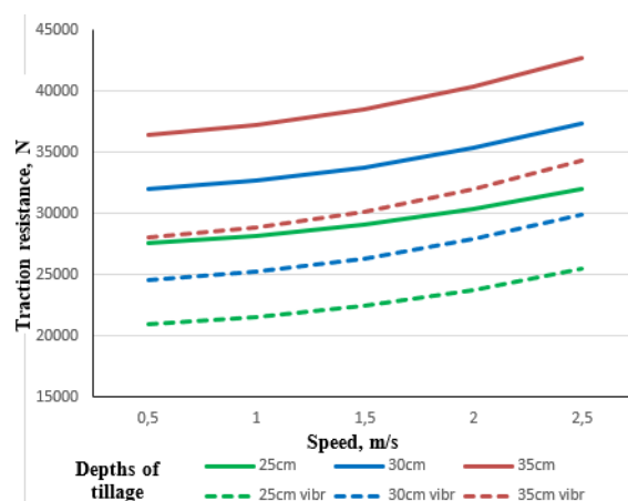
Fig. 2. Dependence of the traction resistance on the speed of movement at different depths of tillage: — theoretical curves without vibrations; - - - theoretical curves with a vibration exciter.
