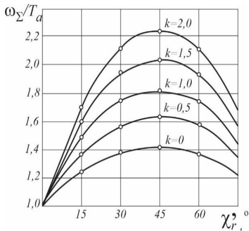
Fig. 3. Dependence of the ratio (\omega_\Sigma)/Ta on the auxiliary setting angle \chi_r'
