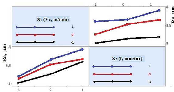
Fig.6. Influence of the factors cutting speed – Vc and feed rate -f to the roughness of the surface.
