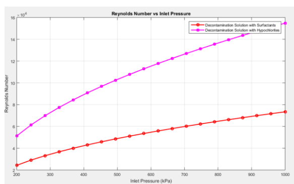
Fig. 4. Relationship between the Reynolds number and the inlet pressure.
