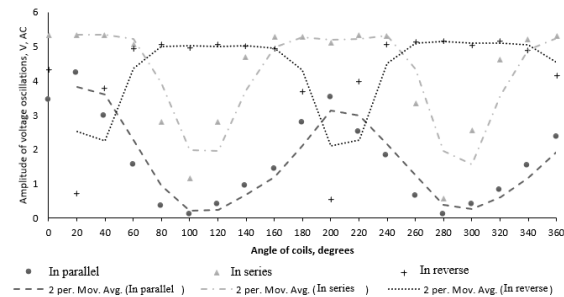
Fig. 8. Dependence of the amplitude of voltage fluctuations on the angle between the coils under load.
