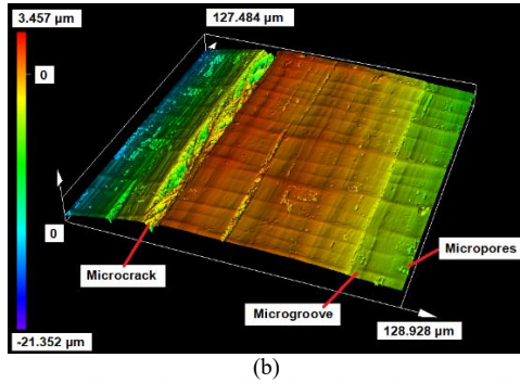
Fig. 7. Sample 1 under magnification of 113 times (a) and 2255 times (b).
