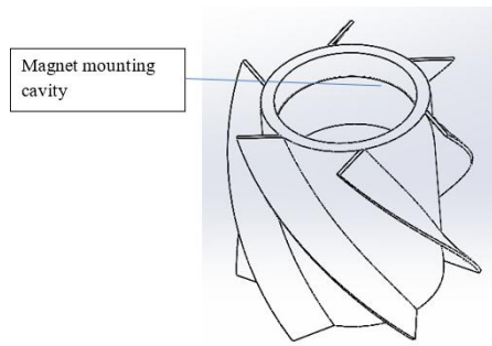
Fig. 1. Impeller used in the experiment.
