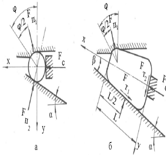
Fig. 1. Loading of the deforming element: a) ball; b) roller.
