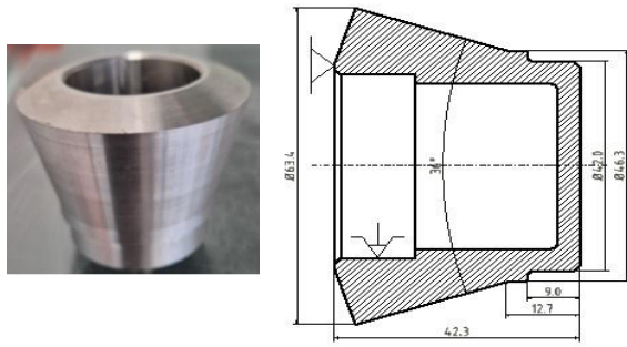
Fig. 2. Machined workpiece
