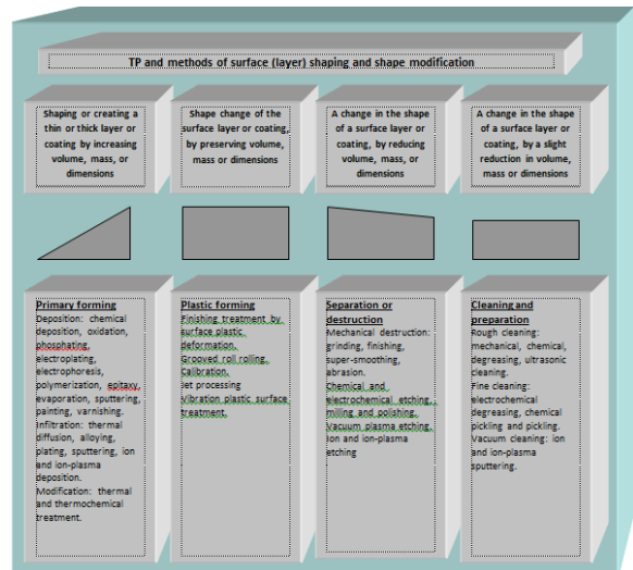
Fig. 5. TP and methods of surface (layer) forming
