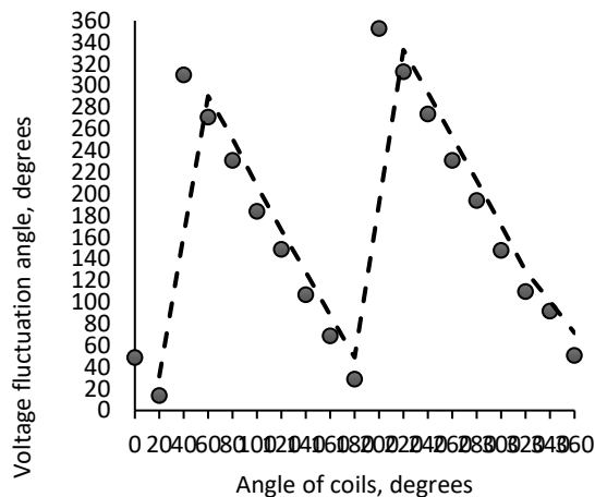
Fig. 3. Dependence of the phase of the electric signal on the angle of the coils.
