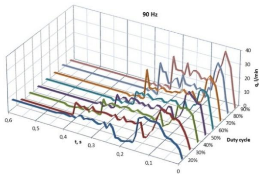
Fig. 14. Variation of the flow rate entering the electropneumatic positioning system.
