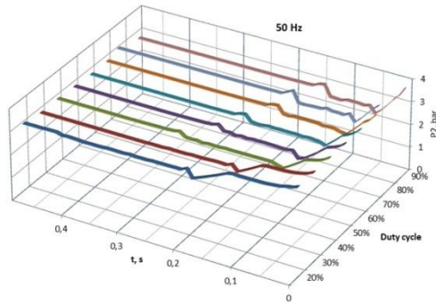
Fig. 9. Pressure washout in the right chamber of the pneumatic cylinder at a frequency of 50 Hz and a different duty cycle.
