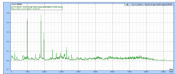
Fig. 6-b. Azimuth thruster oscillation spectrum port side horizontal
