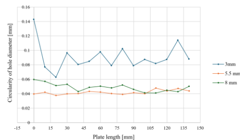
Fig. 8. Dependence of circularity of perforated SS304 stainless steel plates on plate length (perforated plates dimensions - length: 140 mm, width: 25 mm, thickness: 1 mm. Hole diameter: 3 to 8 mm).
