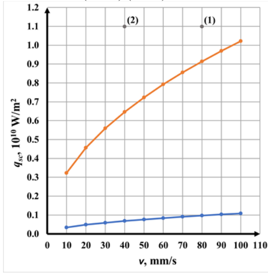
Fig. 2. Graphs of the dependence of the critical power density of melting and evaporation on the speed for AISI 316 steel for the laser cutting process
