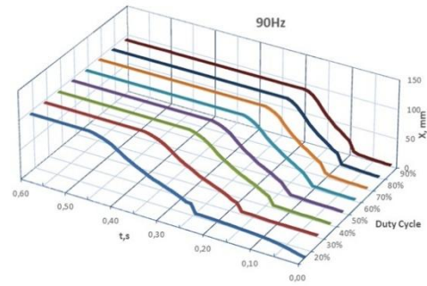
Fig. 11. Displacement of the rod of the pneumatic cylinder at a frequency of 90 Hz and different duty cycle.
