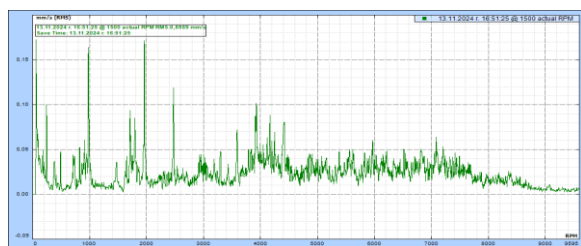
Fig. 6-a. Azimuth thruster oscillation spectrum port side vertical
