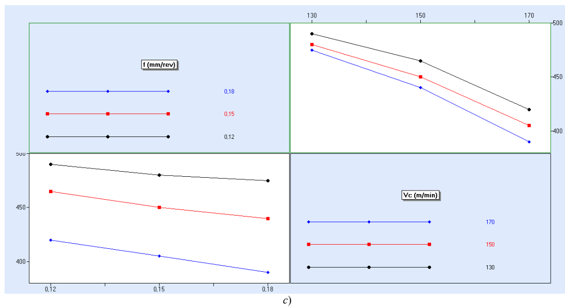
Fig. 5 Visualisation of the influence of the feed f and cutting speed V_c on the tool lifetime of machining with carbide inserts: a - CCMT09T304-F1 TP2501 of a company SECO; b - CCMT09T304-MP of a company PALBIT; c - CCMT09T304-F3M IC807 of a company ISCAR
