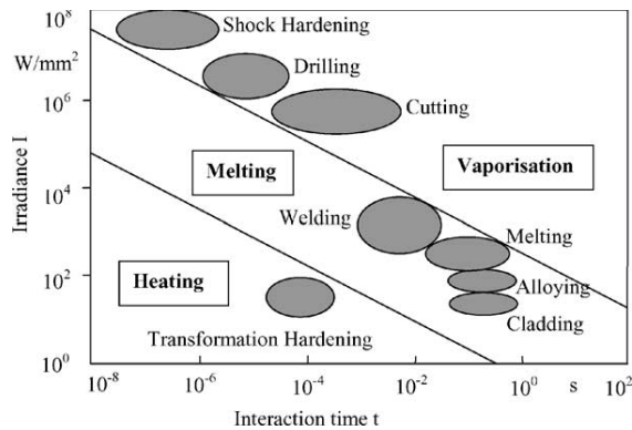
Fig.1. Possible industrial applications of lasers at different interactions of laser radiation with matter [5].
