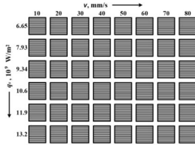
Fig. 2. Designed matrix of the experiments for laser marking of copper samples.
