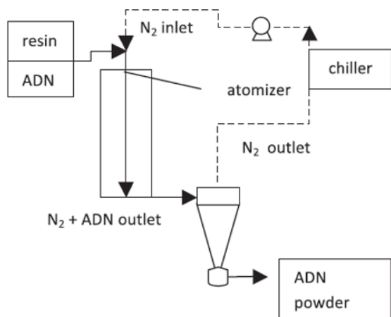
Fig. 3. The spray dryer technique.
