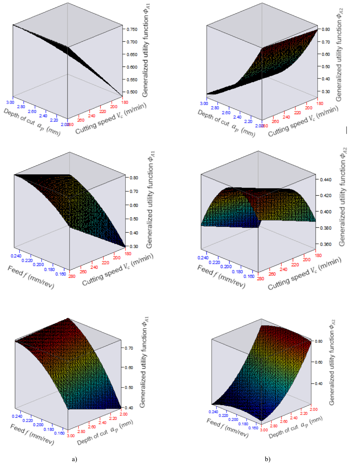
Fig. 3. Graphical visualization of the generalized utility function models for CNC turning: (a) arithmetic mean generalized utility function \phi_{A1} with weighting coefficients w_1 = 0.2 ; w_2 = 0.8 ; (b) arithmetic mean generalized utility function \phi_{A2} with weighting coefficients w_1 = 0.8 ; w_2 = 0.2 .
