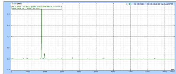
Fig. 4-b. The spectra of the vibrations of the driving bevel gear horizontal
