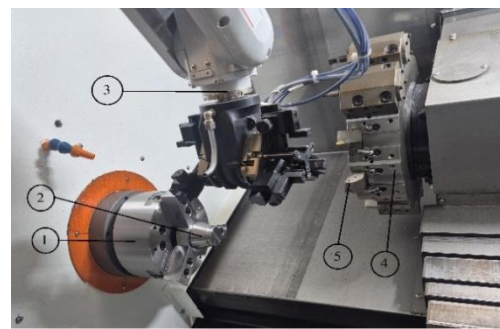
Fig. 1. Workspace of a HARRIS C400 CNC lathe with robotic power supply (1 – chuck; 2- workpiece; 3 - station for robotic power supply Mitsubishi robopro DR800; 4 – turret head; 5 – cutting tool)
