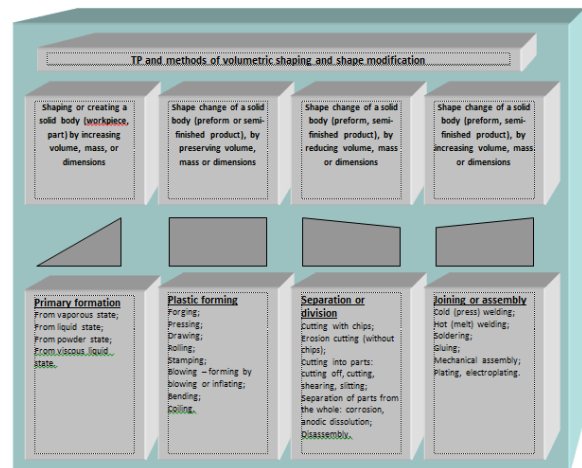
Fig. 4. TP and volumetric forming methods
