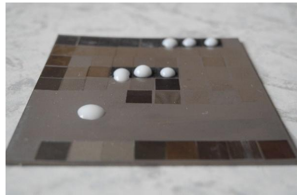
Fig. 2. Laser processing of AISI 316L stainless steel blank piece.
