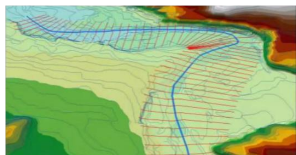
Fig. 4. Determination/extraction of cross section profiles for hydraulic calculations from a digital terrain model
