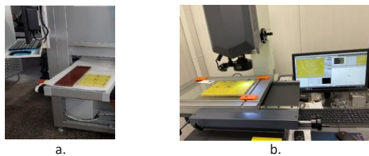
Fig. 3 Equipment, a – marking, b - measuring
