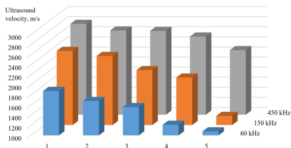
Fig. 7. Changes in ultrasound velocity in perforated plates depending on the specific degree of perforation (1 - 0; 2 - 7.1%, 3 - 12.6%, 4 - 23.8%, 5 - 50.3%) for three ultrasound frequencies (60, 150 and 450 kHz).
