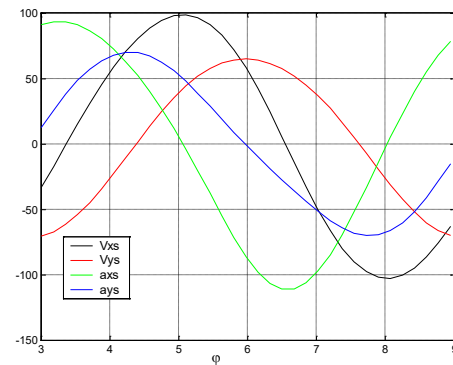
Fig.7. The linear velocities and linear accelerations of the centers of gravity of the initial unit.
