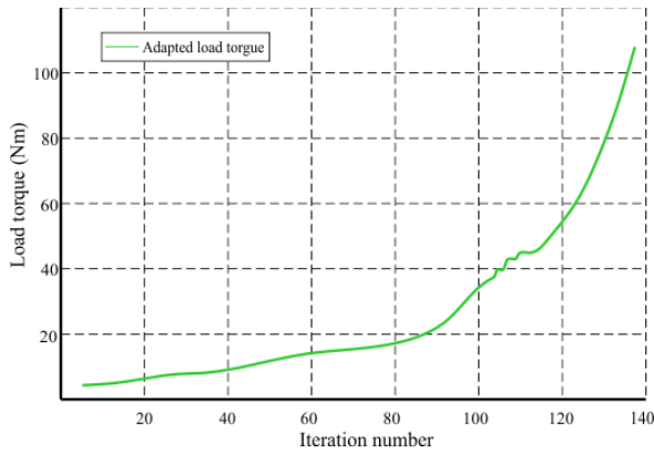
Fig. 3. Adaptive estimation of external load moment by stochastic gradient method (SGD).
