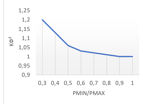
Fig. 1. Dependence of the form factor and limits of variation of electrical loads.
