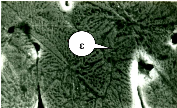
Fig.5. Location of the \epsilon phase along the iron grain boundaries
