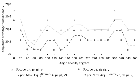
Fig. 4. The dependence of the amplitude of voltage fluctuations on the mutual angle of the coils.
