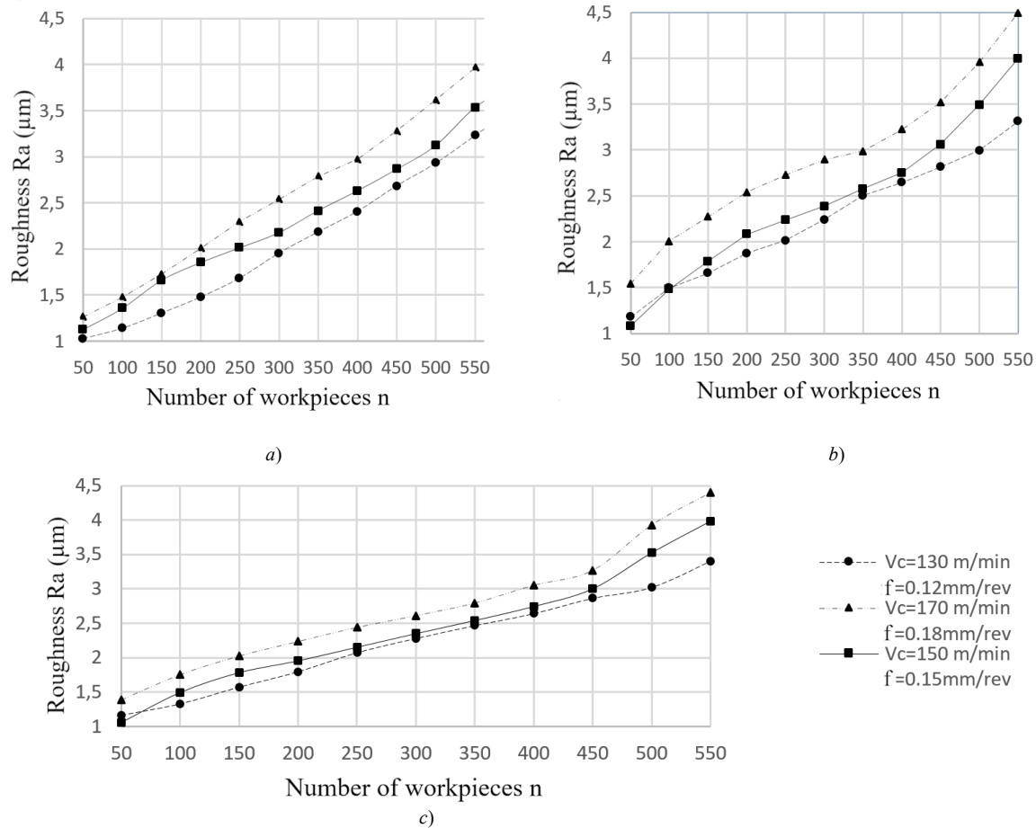
Fig. 3 Variation of roughness depending on the number of machined workpieces in turning with replaceable carbide inserts: a - CCMT09T304-F1 TP2501 of a company SECO; b - CCMT09T304-MP of a company PALBIT; c - CCMT09T304-F3M IC807 of a company ISCAR.
