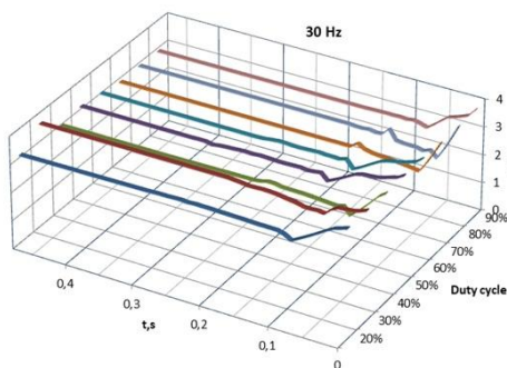
Fig. 5. Pressure washout in the right chamber of the pneumatic cylinder at a frequency of 30 Hz and a different duty cycle.
