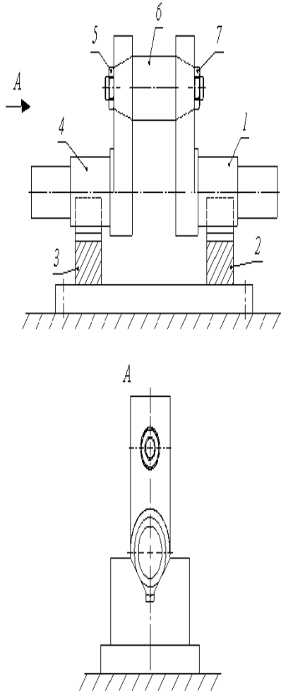
Fig. 1. Device for assembly of crankshaft.
