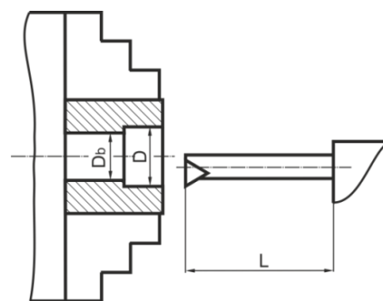
Fig. 2. Experimental scheme ( D_b – diameter of the workpiece; D – diameter of the machine part)
