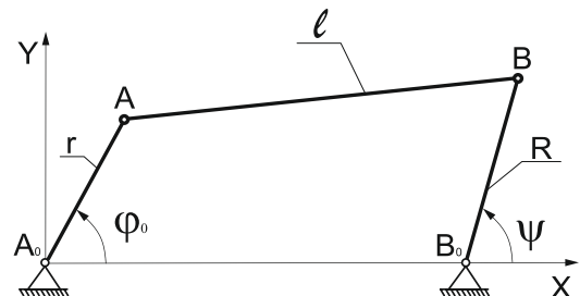
Fig.1 shows a four-bar lever mechanism.
