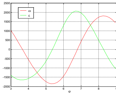
Fig.3 Angular velocity and angular acceleration.
