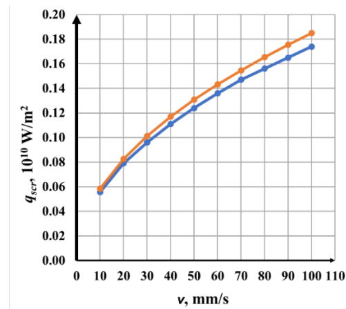
Fig. 5. Graphs of the dependence of the critical melting power density on the speed: blue graph – from numerical experiments and orange graph – from numerical calculations
