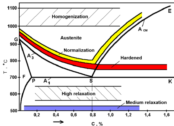
Fig.3. Diagram of surface hardening of steel [25]
