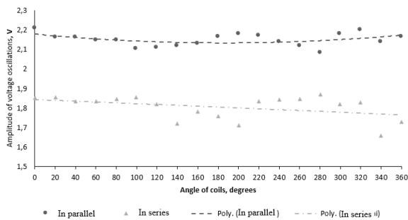
Fig. 15. Curves of the amplitudes of voltage oscillations on the angle of position of the coils at sequential and parallel connections of two sources (with diode bridges and load).
