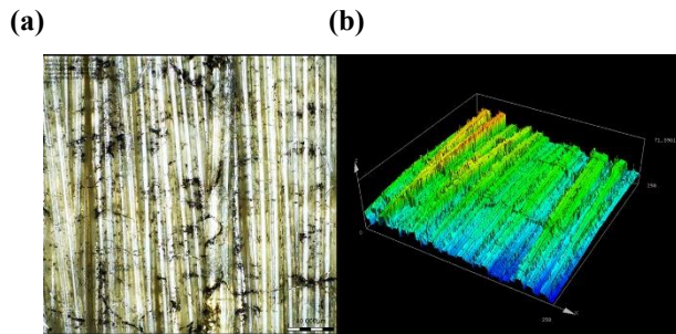
Fig. 4. Surface Morphology of Laser-Marked Graphene-Modified KM2-440 Ballistic Kevlar Fabric at 8.5% Power and 100 mm/s Scanning Speed Showing the Most Pronounced Increase in Surface Roughness Compared to the Unmarked Material.
