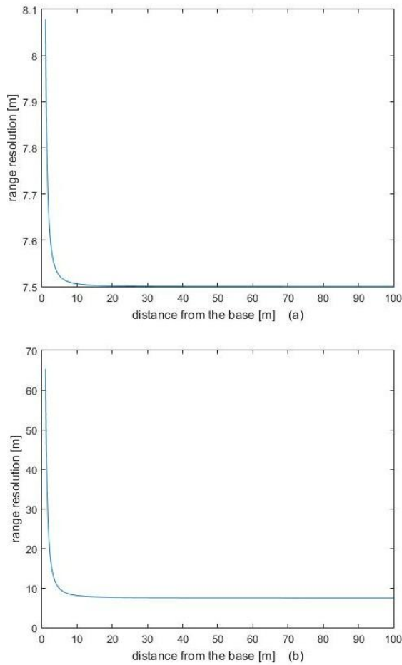
Fig. 3. Range resolution for B=100 [m] a) and B=1000 [m] b).
