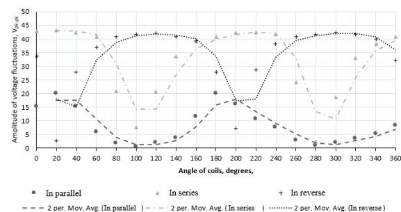
Fig. 6. Change in the voltage amplitude of different connections of two sources from the angle of the coils.
