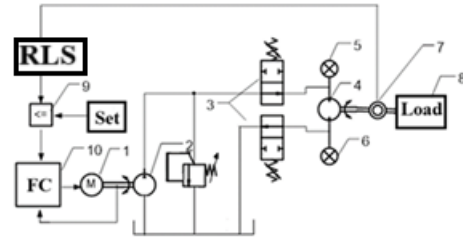
Fig. 1. Schematic diagram of electro-hydraulic drive system.
