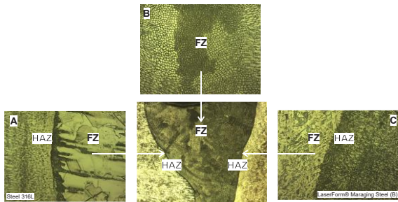
Fig. 2. Weld seam of both materials at x 50 magnification and transition zones at x 500 magnification between: A) 316L steel and weld seam; B) within the weld seam itself and C) weld seam and LaserForm Maraging Steel (B).
