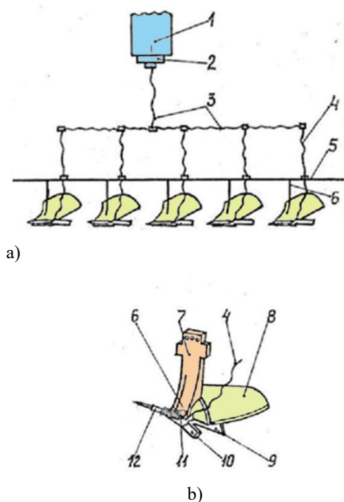
Fig. 1. Scheme of a plough with pneumatic soil looseners: a) general; b) plough body; 1 – tractor pneumatic system; 2 – a mechanism for controlling the degree of loosening of the soil; 3 – common pneumoline; 4 – pneumoline of the plough body; 5 – frame; 6 – plough body; 7 – rack; 8 – shelf; 9 – ploughshare; 10 – field board; 11 – air distribution mechanism; 12 – pneumatic hammer.
