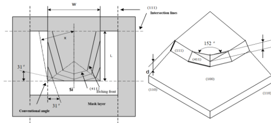
Fig. 4. Principle of conventional corner etching and partial etching of freely vibrating components
