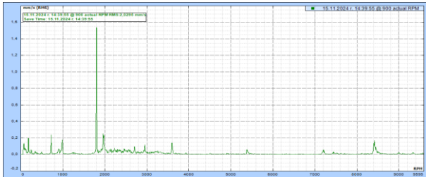
Fig. 4-a. The spectra of the vibrations of the driving bevel gear vertical
