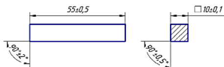
Fig. 1 Geometric dimensions of blanks from CADI and austenitic stainless steel AISI 316L.
