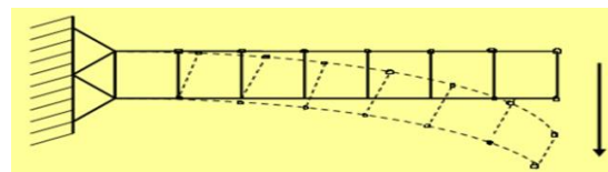
Fig. 14 End elements of a tensioned beam loaded in bending.
