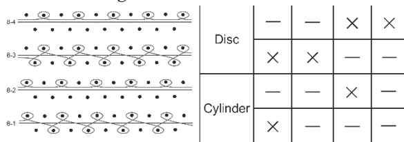
Fig. 8. Fabric-like knit on interlock basis without press elements.
