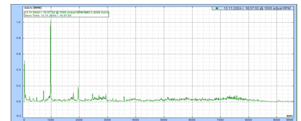
Fig. 7-b Azimuth thruster oscillation spectrum starboard side horizontal
