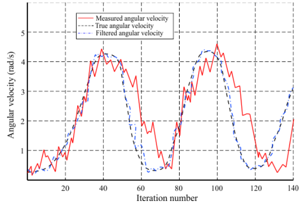
Fig. 2. Comparison of measured, true, and filtered angular velocity estimated by RLS with gradient correction.
