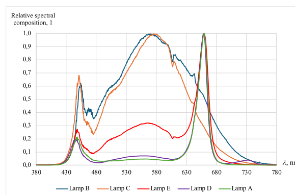
Fig. 1. Relative spectral composition of all 5 used luminaires
