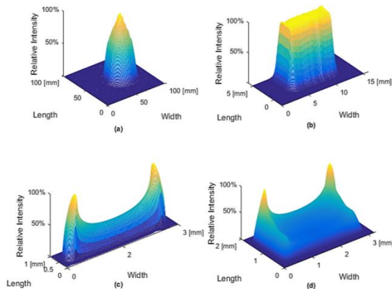
Fig. 8. For laser hardening, four intensity profiles are commonly used. The defocused round top-hat profile (a); the rectangular top-hat profile (b); the intensity profile generated by a harmonic oscillation of a scanning mirror (c) as well as the optimized intensity profile which was calculated by Burger [42].
