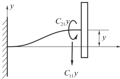
Fig. 5-a. the elastic constants of the cantilever shaft. When specifying a displacement y
