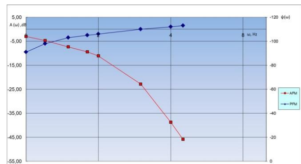
Fig. 4. AFR and PFR at an input signal amplitude of 0.5 V.
