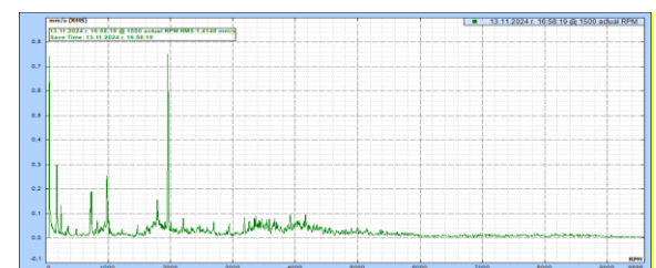
Fig. 7-c Azimuth thruster oscillation spectrum starboard side axial
