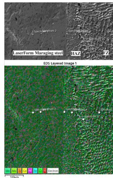
Fig. 4. EDX analysis in HAZ and FZ of weld LaserForm Maraging Steel (B).
