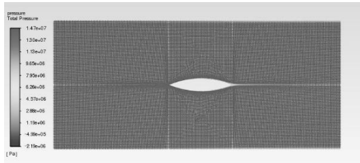
Fig. 6. FOM Simulation for the Pressure.
