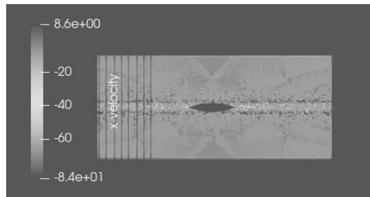
Fig. 7. Reconstructed x-velocity in spatial points.
