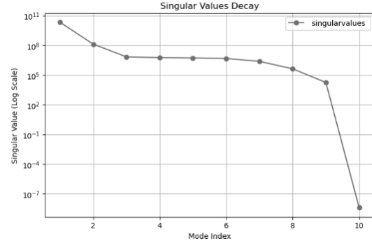
Fig. 2. Singular Values of the 10 snapshots.
