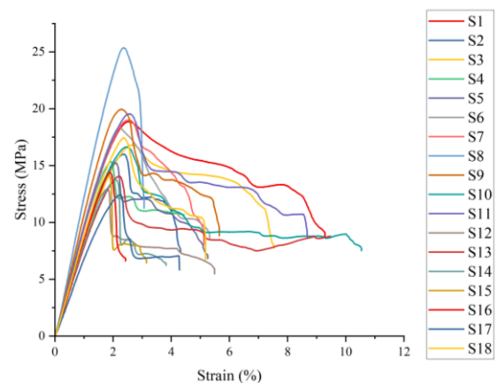
Fig. 3. Representative stress-strain curves for 18-different infill patterns (S1-S18).
