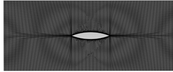
Fig. 1. Mesh Generation of Fluid Domain.
