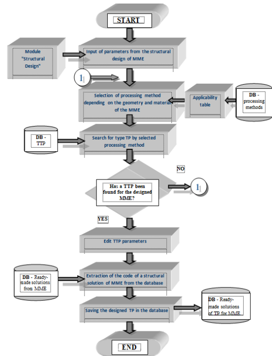
Fig. 3. Flowchart of the algorithm for selecting a technological process (TP) of the automated system "MICROSYS 25"
