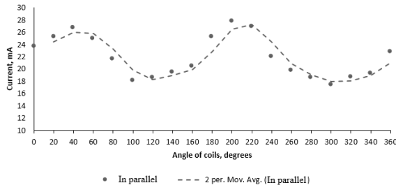
Fig. 14. The dependence of the current generated by two sources connected in parallel on the angle between the coils (with diode bridges and load).
