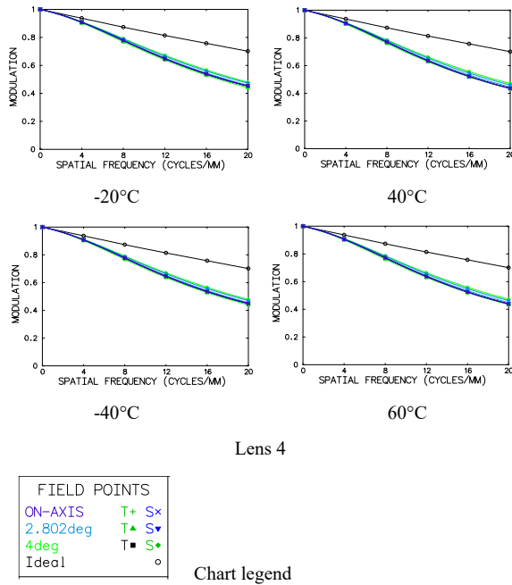
Fig. 3. MTF of lenses for different temperatures.
