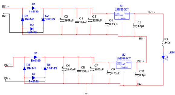
Fig. 9. Principle electrical diagram of the sequential connection of two sources.
