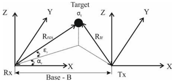
Fig. 1. Geometry of bistatic passive radar.
