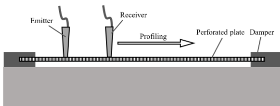
Fig. 4. Layout of ultrasonic measurements on the perforated plate.
