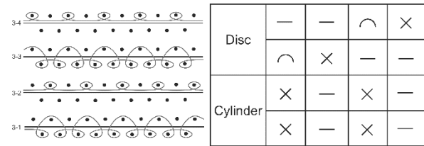
Fig. 3. Fabric-like knit with press elements.
