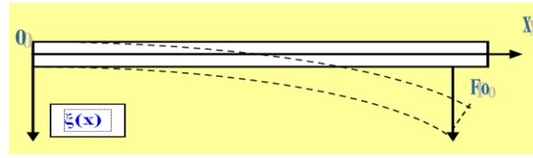
Fig. 11 Diagram of a beam under bending load
