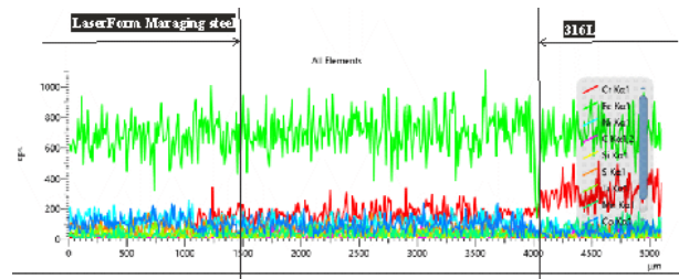
Fig. 3. Line EDX analysis in HAZ and FZ of weld.
