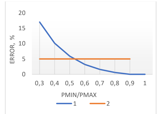
Fig. 2. Dependence of the error and limits of variation of electrical loads - 1 and Limit value - 2.
