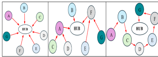
Fig. 5. Star, Mesh and Line topologies (Hub means the gateway)
