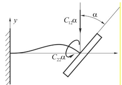
Fig. 5-c the elastic constants of the cantilever shaft. When specifying a displacement \alpha
