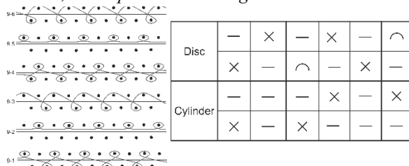
Fig. 9. Fabric-like knit on interlock basis without press elements.
