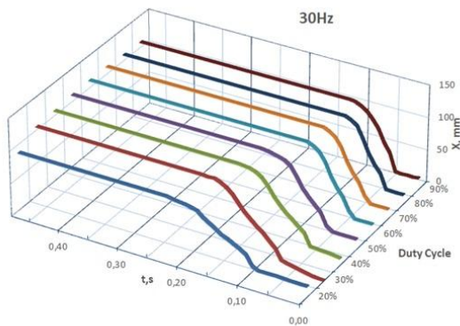
Fig. 3. Displacement of the rod of the pneumatic cylinder at a frequency of 30 Hz and different duty cycle.
