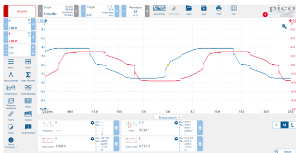
Fig. 10. Oscilloscope showing the changes in the generated voltage fluctuations (with diode bridges and load in the presence of a sequential connection).
