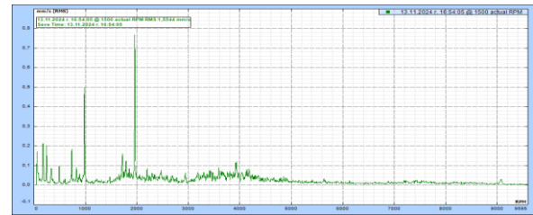
Fig. 6-c. Azimuth thruster oscillation spectrum port side axial
