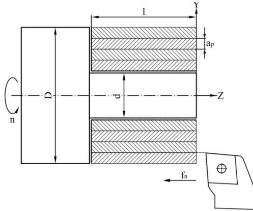
Fig. 3. Multi-pass cylindrical turning .
