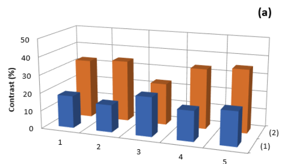
Fig. 6. Contrast Response at Multiple Surface Points on Laser-Marked Matrices (1) and (2).
