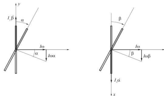
Fig. 4-b. Projection of the kinetic moment along the x and y axes
