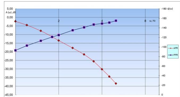
Fig. 3. AFR and PFR at an input signal amplitude of 0.3 V.
