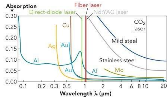
Fig.7. Radiation of laser absorbed varies the wavelength for different metals [40].
