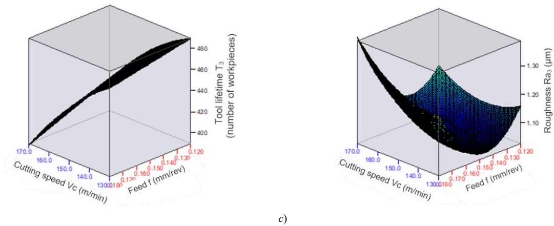
Fig. 4 Graphical dependences of the tool lifetime of the inserts and the roughness of the machined surfaces depending on the feed f (mm/rev) and cutting speed V_c (m/min) (a - CCMT09T304-F1 TP2501 of a company SECO; b - CCMT09T304-MP of a company PALBIT; c - CCMT09T304-F3M IC807 of a company ISCAR)
