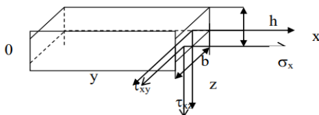
Fig. 3. Stresses expressing external forces on a beam
