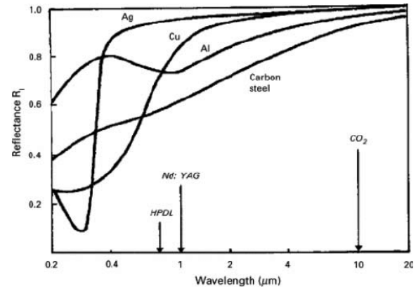
Fig.5. Reflectivity as a function of wavelength for various materials.[28].
