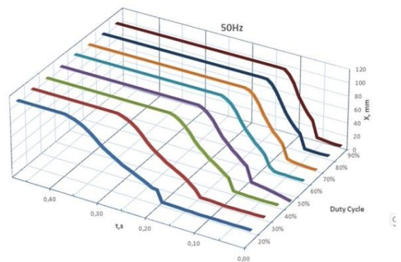
Fig. 7. Displacement of the rod of the pneumatic cylinder at a frequency of 50 Hz and different duty cycle.
