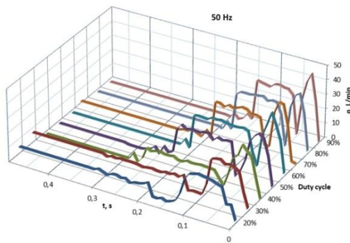
Fig. 10. Variation of the flow rate entering the electropneumatic positioning system.
