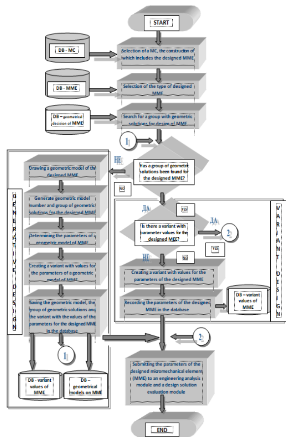
Fig. 2. Block diagram of the geometric modeling algorithm from the automated system "MICROSYS 25"
