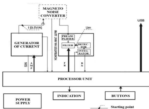
Fig. 1. Block diagram of the device for measuring EBN.
