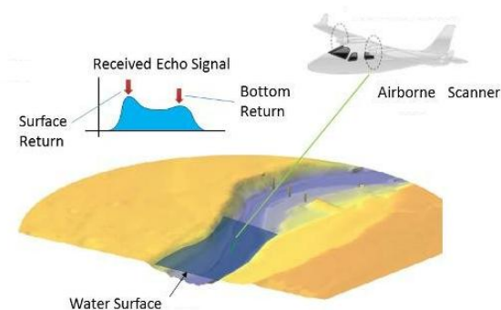
Fig. 7. Laser scanning
