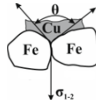
Fig.6. Scheme of the formation of the bilateral angle - \theta , of the solid (Fe) / liquid (Cu) phase boundary
