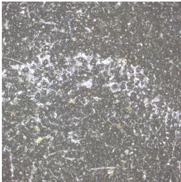
Fig. 7. Milk solids (white) in laser made hydrophobic surface structure.
