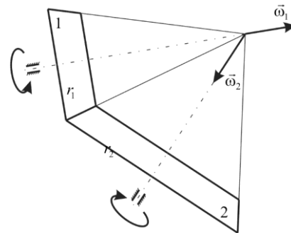
Fig. 1. The influence of geometric eccentricity on the vibrations of bevel gears
