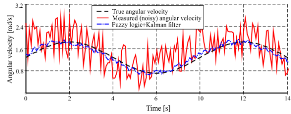
Fig. 3. Fig. 3: Angular velocity change with optimized covariance matrices Q and R in EKF.
