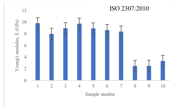
Fig. 6. Comparison graph of Young's modulus values of the ten samples.
