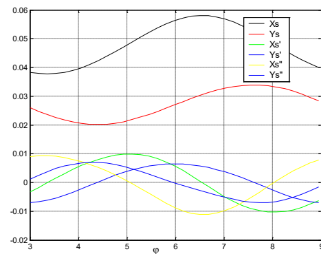
Fig.6 The coordinates of the centers of gravity of units 1, 2 and 3.
