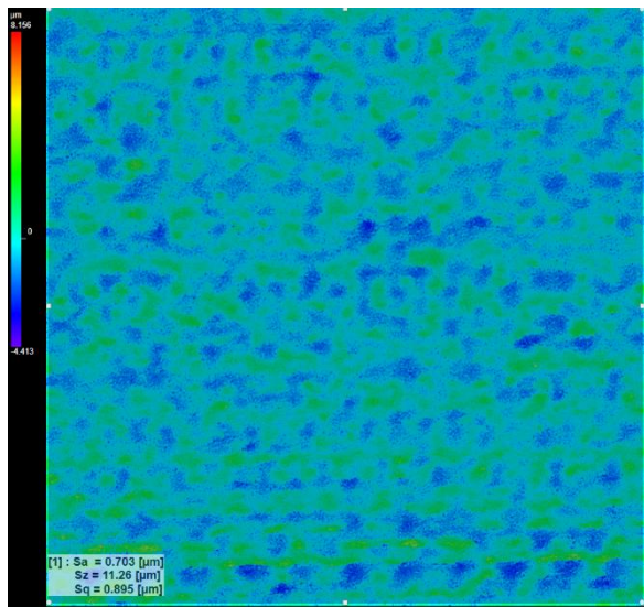
Fig. 3. Laser made hydrophobic surface “heat map” and software calculated roughness parameters.
