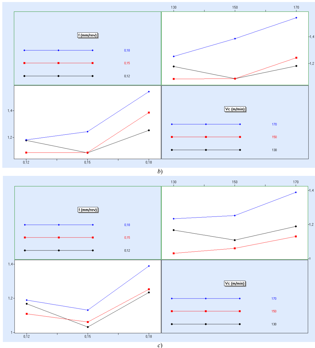
Fig. 6 Visualisation of the influence of the feed f and cutting speed V_c on the roughness of machining with carbide inserts: a - CCMT09T304-F1 TP2501 of a company SECO; b - CCMT09T304-MP of a company PALBIT; c - CCMT09T304-F3M IC807 of a company ISCAR.
