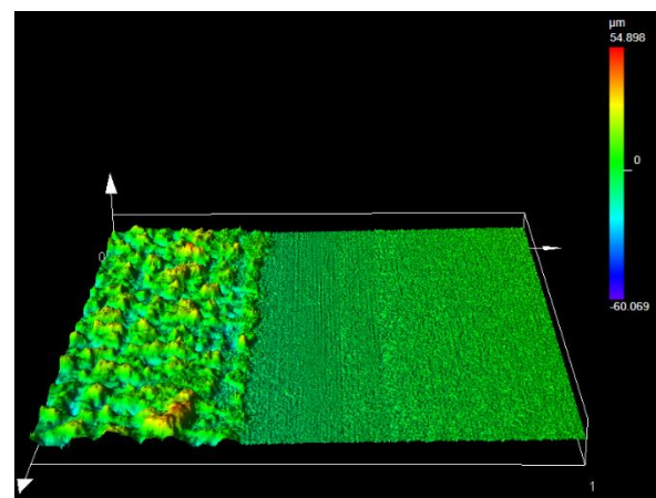
Fig. 10. Microscopic structure comparison of laser “polished” (right) and laser made hydrophobic surfaces (right).
