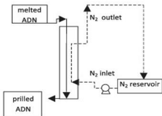
Fig. 1. The schematics of Prilling Tower technique for production of ammonium dinitramide granules.
