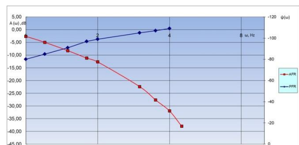
Fig. 5. AFR and PFR at an input signal amplitude of 0.7 V.
