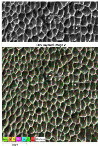
Fig. 5. EDX analysis in FZ of weld
