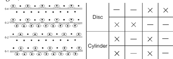
Fig. 6. Fabric-like knit on interlock basis with press elements.
