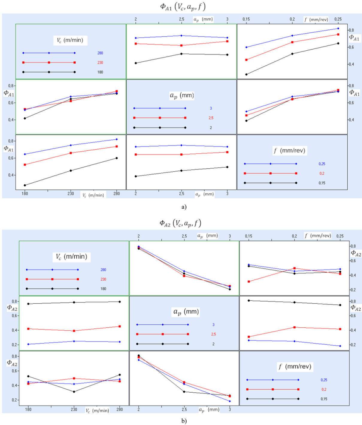
Fig. 4. Interaction plots for the generalized utility function models for CNC turning: (a) arithmetic mean generalized utility function \Phi_{A1} with weighting coefficients w_1 = 0.2 ; w_2 = 0.8 ; (b) arithmetic mean generalized utility function \Phi_{A2} with weighting coefficients w_1 = 0.8 ; w_2 = 0.2 .
