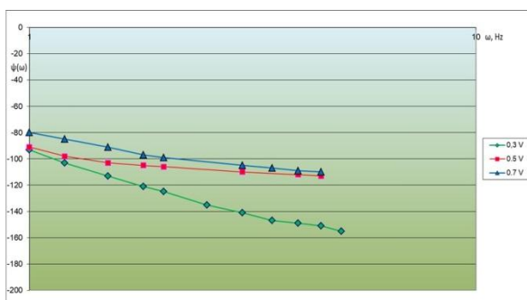
Fig. 7. PFR at input signal amplitudes of 0.3 V, 0.5 V, and 0.7 V.
