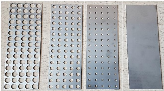
Fig. 3. Perforated stainless steel SS304 plates. Length: 140 mm, width: 25 mm, thickness: 1 mm. Hole diameter: 3 to 8 mm. Total perforation area: 0% to 50%.
