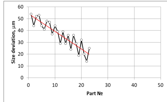
Fig. 4. Scatter diagram of the process of clean boring of a batch of cylindrical bushings with the application of a statistical method for dimensional sub-tuning
