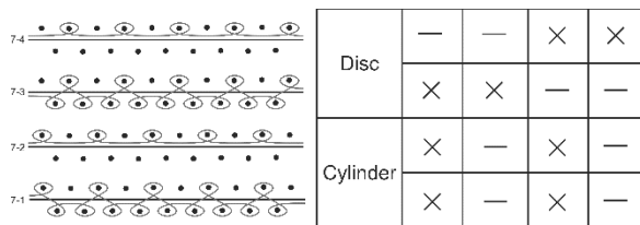
Fig. 7. Fabric-like knit on interlock basis with press elements.
