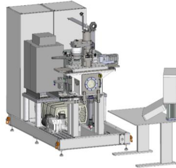
Fig. 1. Evobeam Cube 400 welding unit manufactured by Evobeam.
