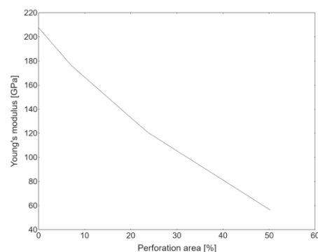
Fig. 6. Dependence of Young's modulus of perforated SS304 stainless steel plates on perforation (perforated plates dimensions of Length: 140 mm, width: 25 mm, thickness: 1 mm. Hole diameter: 3 to 8 mm. Total perforation area: 0% to 50%).
