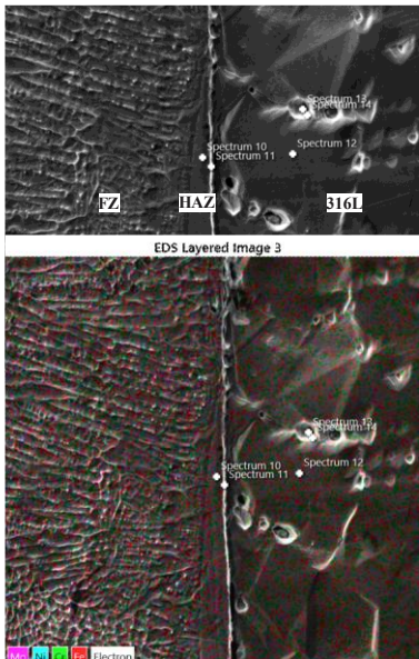
Fig. 6. EDX analysis in HAZ and FZ of weld of AISI 316L Stainless steel.
