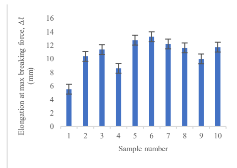
Fig. 4. Comparison graph of the values of elongation at maximum breaking force of the ten samples.
