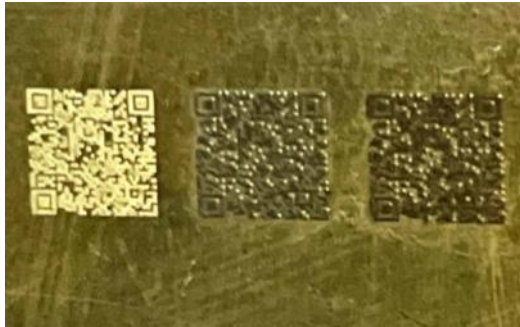
Fig. 9. Obtained QR codes on brass surface – starting from left end, white (light), grey (middle) and dark (right end) marking, respectively.
