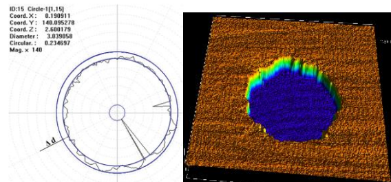
Fig. 5. Perforation profile with 3 mm diameter in SS304 steel plate and enlarged perforation 3D profile.
