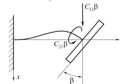
Fig. 5-d. the elastic constants of the cantilever shaft. When specifying a displacement \beta
