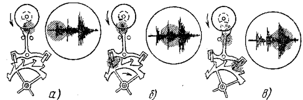
Fig. 2. Schematics of the oscillator beats
