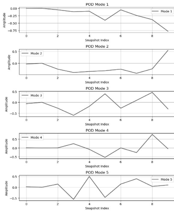
Fig. 4. POD Modes Rank = 5.
