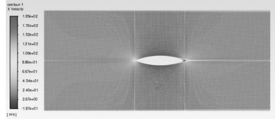
Fig. 8. FOM of x-velocity.
