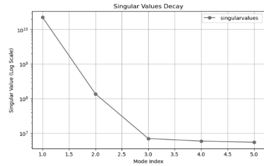
Fig. 3. Rank=5 Truncated Singular Values.
