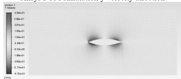
Fig. 10. FOM of Y- velocity.
