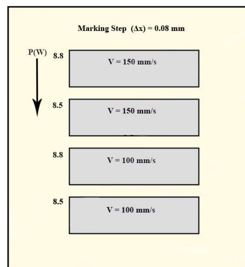
Fig. 3. Laser marking schematics of GRAPHENE-MODIFIED KM2-440 BALLISTIC KEVLAR FABRIC.
