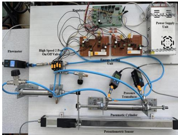
Fig. 1. Demonstration Research Test Stand.
