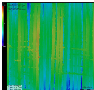
Fig. 9. High-Contrast Surface Modification on Graphene-Modified Kevlar (Matrix 2).
