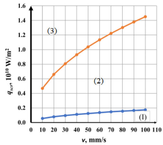
Fig. 4. Graphs of the dependence of the critical power density of melting (blue graph) and evaporation (orange graph) on the speed
