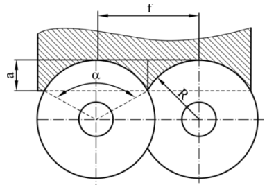
b. when turning by a knife with a round plate
