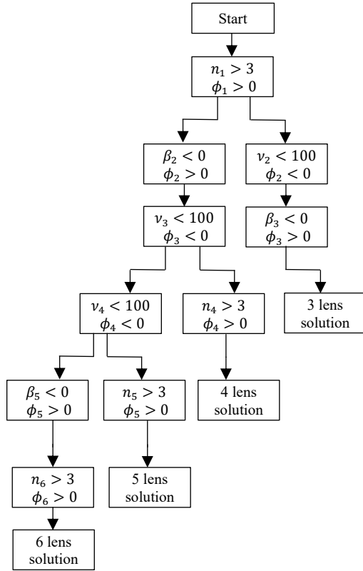
Fig. 2. Block diagram for selection of materials for passive athermalization of an IR lens.
