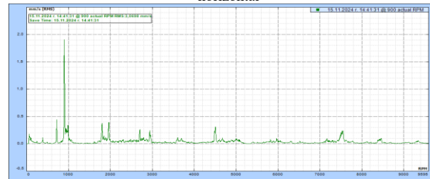
Fig. 4-c. The spectra of the vibrations of the driving bevel gear axial
