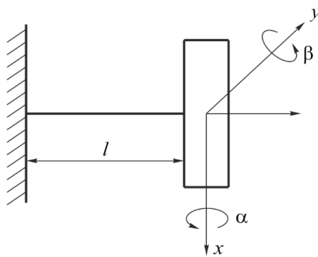
Fig. 1. The propeller shaft is of the cantilever type
