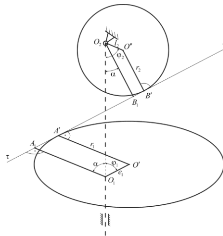
Fig. 1. The influence of geometric eccentricity on the vibrations of bevel gears
