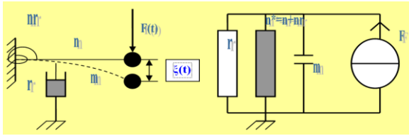
Fig. 10 Modified model of the tensioned beam model
