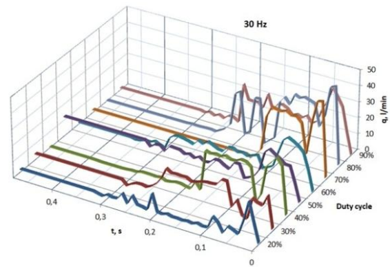
Fig. 6. Variation of the flow rate entering the electropneumatic positioning system.
