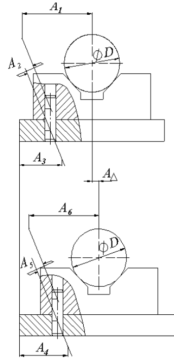
Fig. 2. Dimensional chain.
