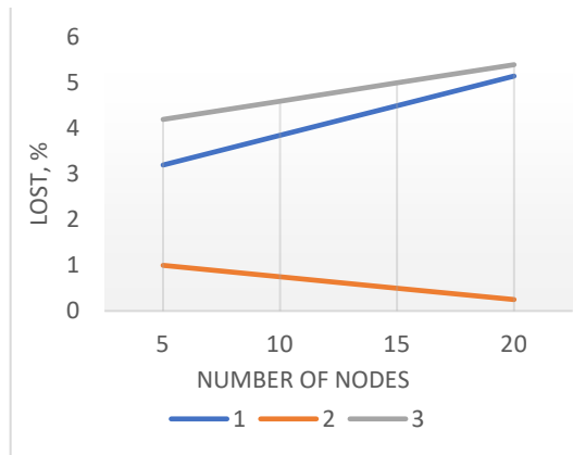
Fig. 3. Average values of power losses in a distribution network: 1 – main component; 2 – dispersion ingredient; 3 – total value.
