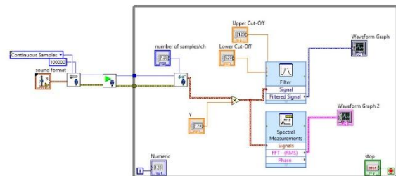
Fig. 3. Block diagram of the measuring system in LabVIEW
