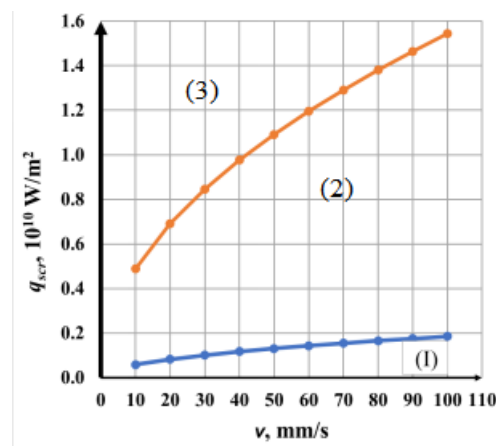
Fig. 2. Graphs of the dependence of the critical power density of melting (blue graph) and evaporation (orange graph) on the speed.
