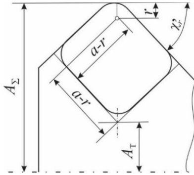
Fig. 1. Dimensioning square insert
