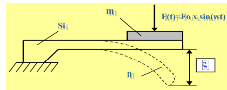
Fig. 5 Technical model of the tensioned beam \xi
