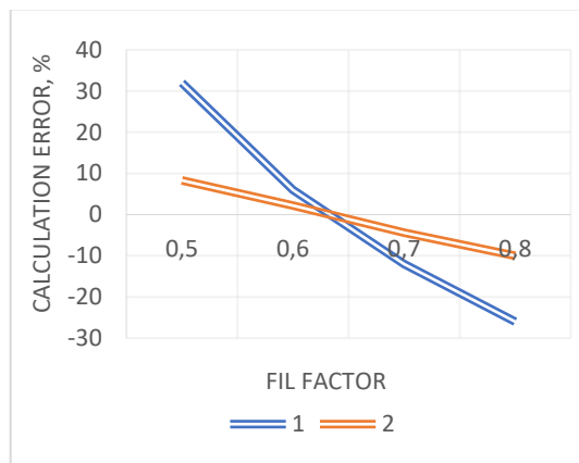
Fig. 4. Error in determining the electricity losses depending on the filling factor: 1 – with the fictitious duration method; 2 – with a probabilistic approach.
