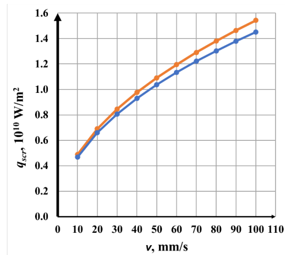
Fig. 6. Graphs of the dependence of the critical power density of evaporation on the speed: blue graph – from numerical experiments and orange graph – from numerical calculations
