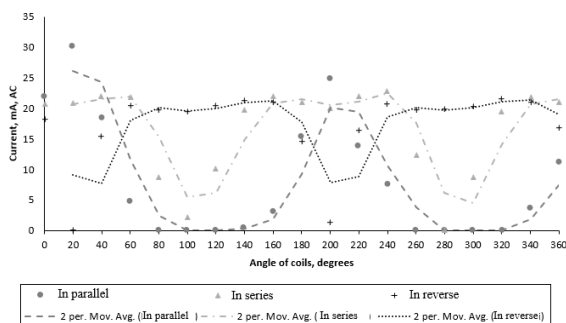
Fig. 7. The dependence of electric current on the angle between the coils under load.
