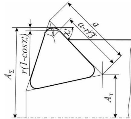
Fig. 4. Dimensioning triangle insert
