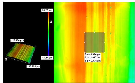
Fig. 8. Example of roughness measurement (sample no. 8).
