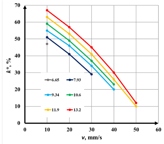
Fig. 5. Graphs of the dependence of contrast on speed for dark marking.
