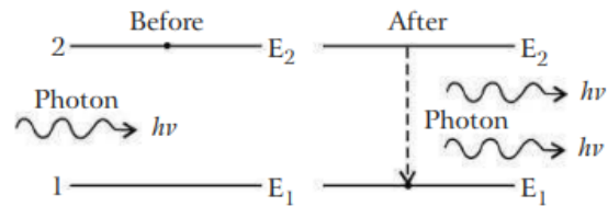
Fig. 2. Stimulated or induced emission. Source: Physical Optics and Lasers by R.K. Agrawal
