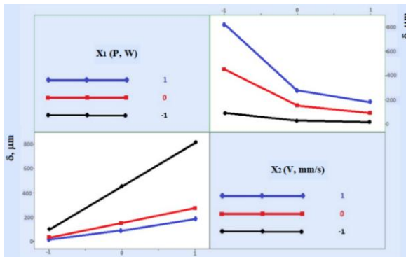
Fig.7. Dispersion analysis of Y_2 = f(X_1, X_2) .
