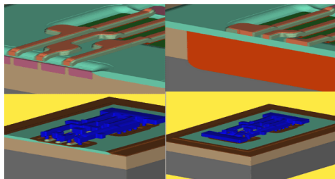
Fig. 15 Simulation of technology of a tensioned beam loaded in bending
