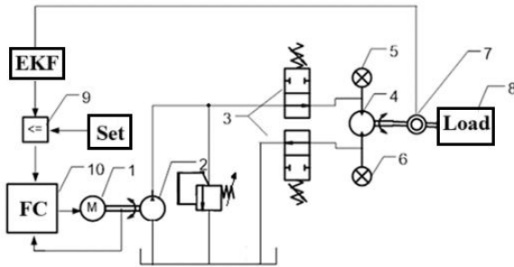
Fig. 1. Structural diagram of the electro-hydraulic system.
