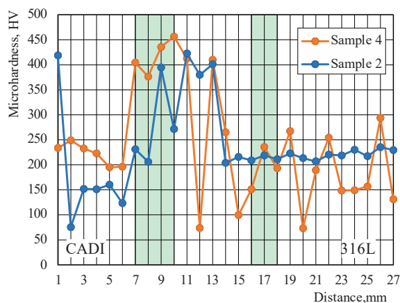
Fig. 4 Measured microhardness of electron beam welded samples with Beam current I_b=20\text{mA} .
