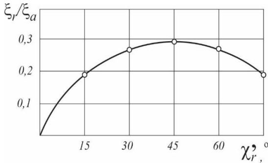
Fig. 2. Dependence of the ratio of the transmission coefficients \xi_a and \xi_r on the auxiliary setting angle
