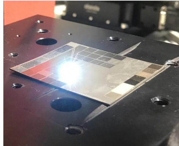
Fig. 1. Laser processing of AISI 316L stainless steel blank piece.
