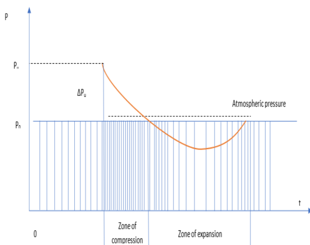
Fig. 4. Pressure Variation Over Time at a Point in the Atmosphere Through Which the Shock Wave Passes.
