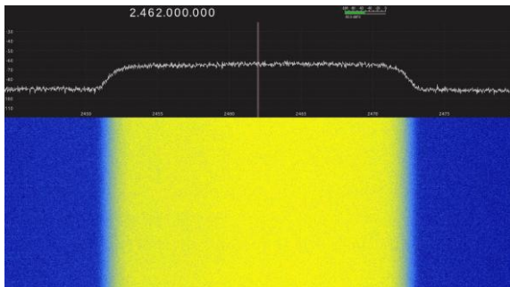
Fig. 10. The barrage jamming on the Wi-Fi radio connection.
