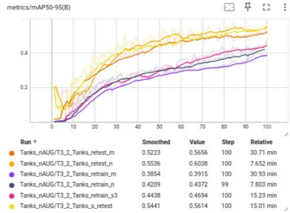
Fig. 6. mAP50 for Re-train vs Pre-trained
