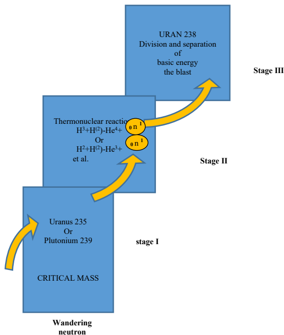
Fig. 2. Scheme of the fusion reaction.
