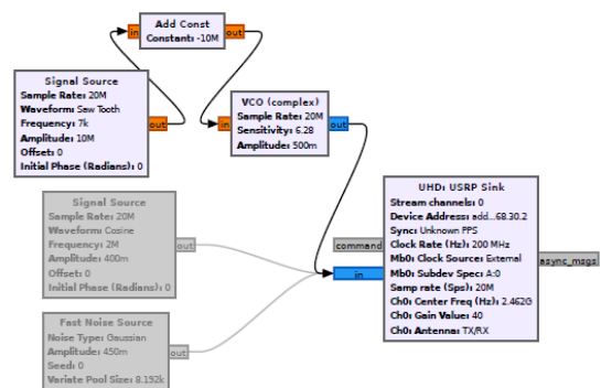
Fig. 8. GNU Radio Framework flowgraph of SDR for EA.
