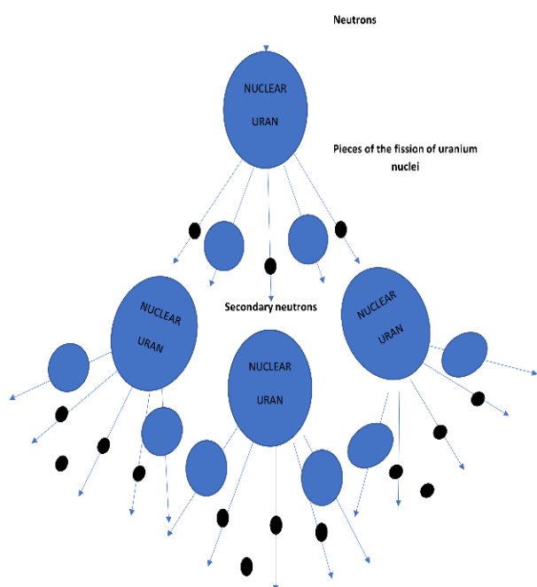
Fig. 1. Diagram of the Chain Reaction.
