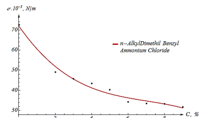
Fig. 4. Surface Tension versus Concentration of n-Alkyl Dimethyl Benzyl Ammonium Chloride.
