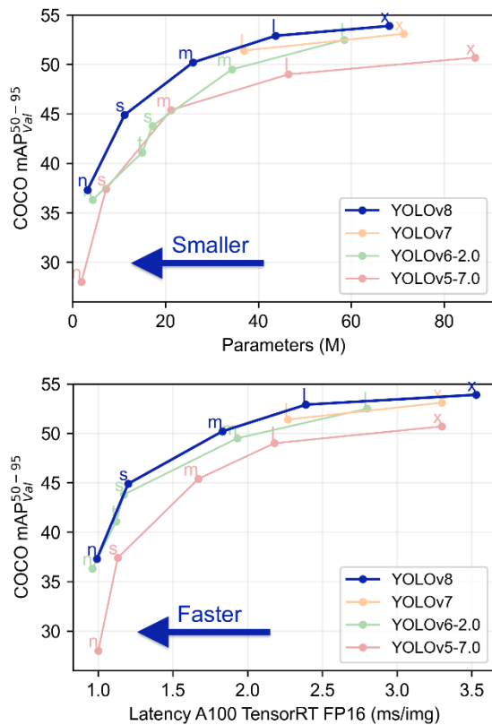
Fig. 1. Comparison of YOLO performance across versions [8]
