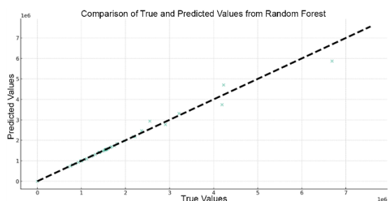
Fig. 1. Graph: Comparison of true and predicted values from Random Forest
