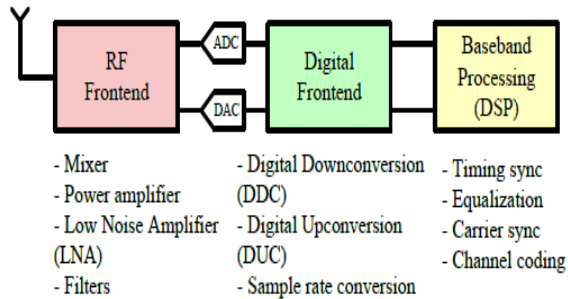
Fig. 4. Software-defined radio architecture
