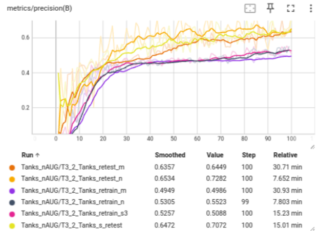
Fig. 7. Precision for Re-train vs Pre-trained
