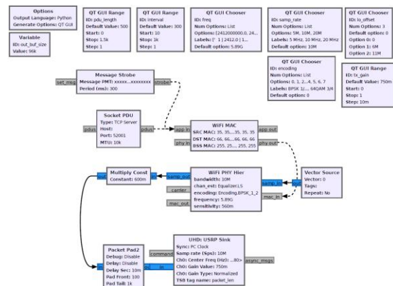
Fig. 12. GNU Radio Framework flowgraph of SDR Wi Fi transmitter performing ED.
