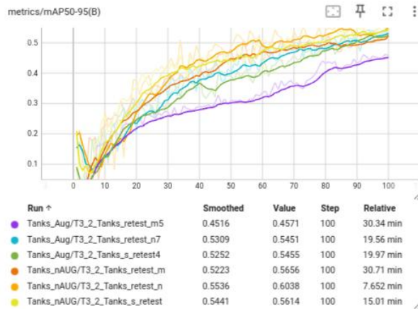
Fig. 9. mAP50-95 for all 3 models with and without augmentations
