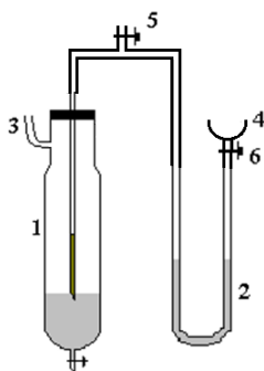
Fig. 1. Schematic of an experimental set-up for determining the surface tension by the "Maximum pressure when blowing a bubble from the capillary" method.
