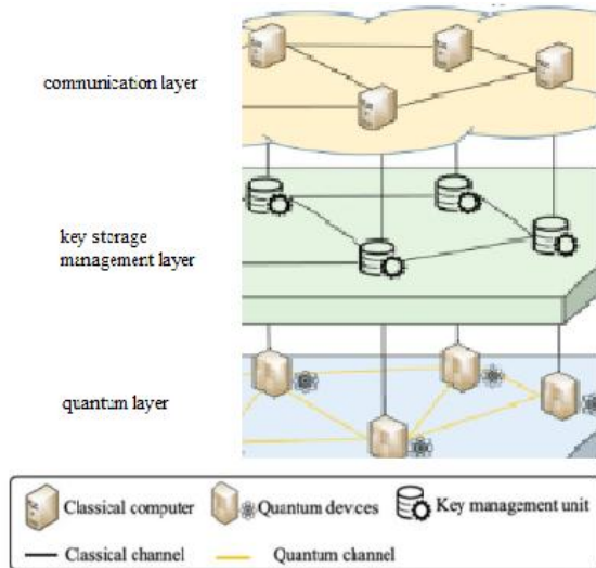
Fig.5. Communication scheme on layers on the QKD network.
