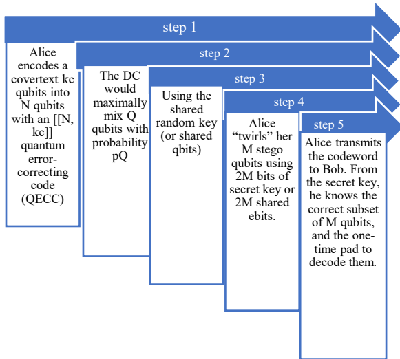
Fig. 2 Visualization quantum steganography protocol.
