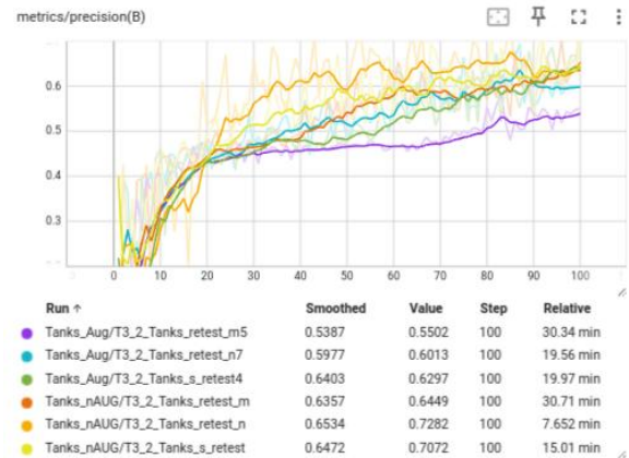
Fig. 10. Precision for all 3 models with and without augmentations
