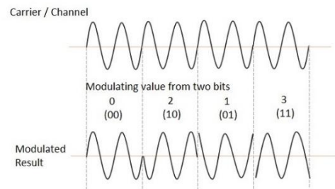
Fig. 3. QPSK waveform.
