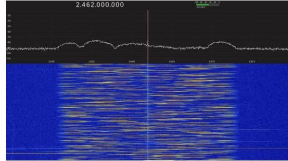
Fig. 11. The scanned jamming on the Wi-Fi radio connection.
