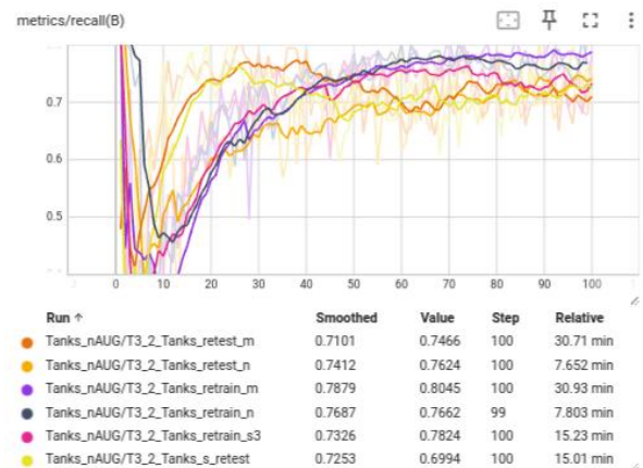
Fig. 8. Recall for Re-train vs Pre-trained
