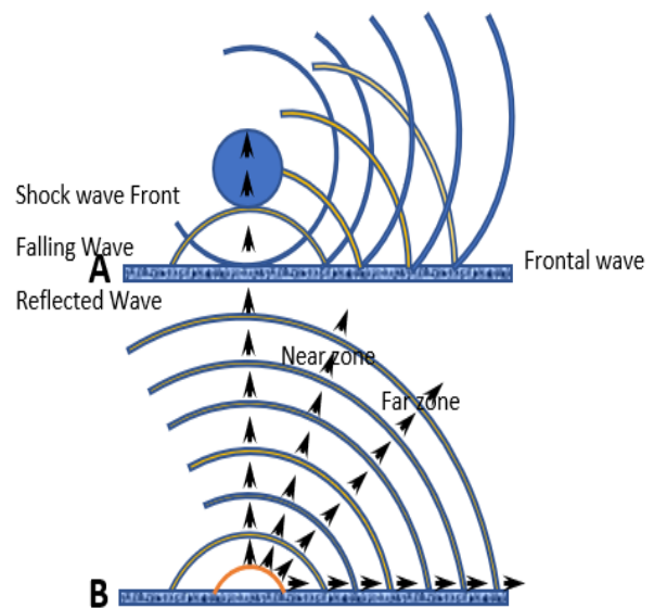
Fig. 3. Diagram of the Formation and Propagation of the Shock Wave (A – Air Explosion; B – Surface Explosion).
