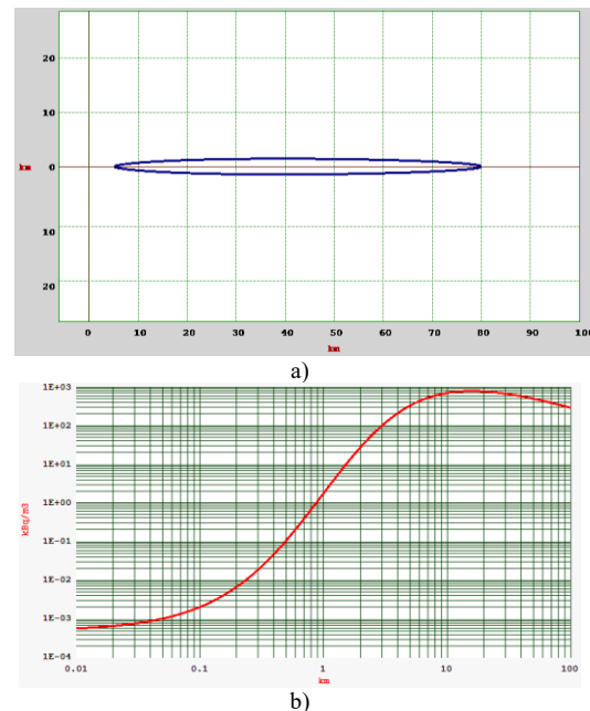
Fig. 2. Dependence of terrestrial radioactive deposition on the center of the accident accompanied by fire in vertical stability class A: a) areas of radioactive deposition b) graphical dependence on concentration and distance
