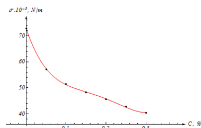
Fig. 5. Surface Tension versus Concentration of DV-2.
