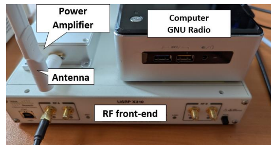
Fig. 7. Implementation of SDR for EA.
